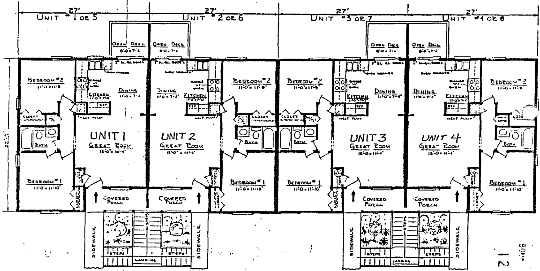
FRANKLIN SQUARE BUILDING B FIRST FLOOR LEVEL
