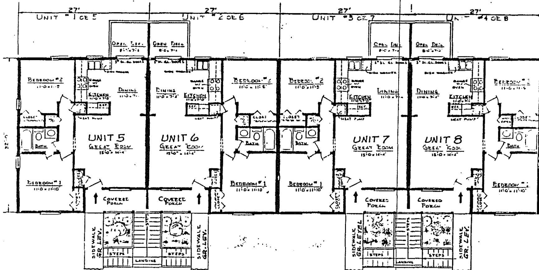
FRANKLIN SQUARE BUILDING A SECOND FLOOR LEVEL
