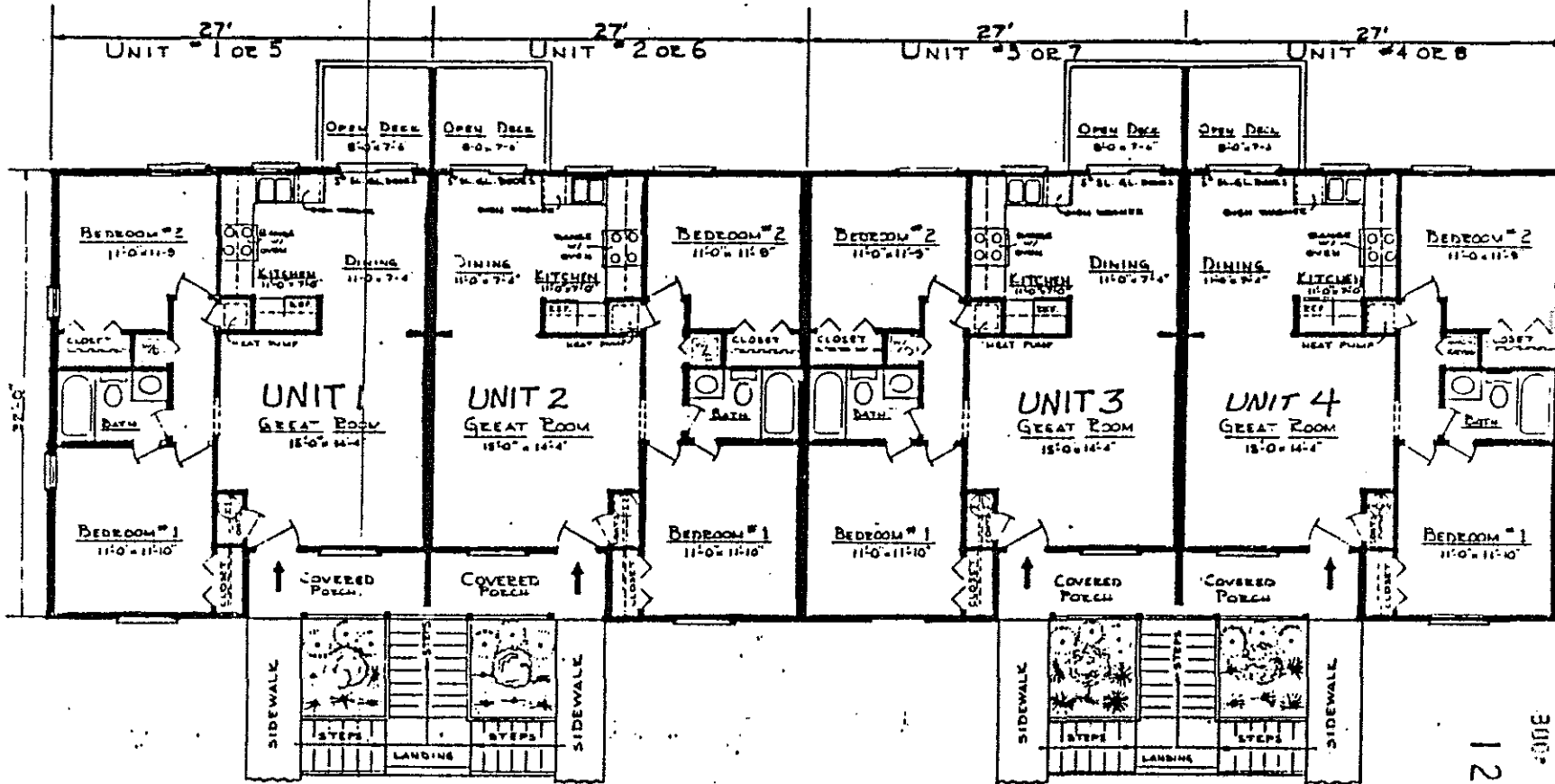
FRANKLIN SQUARE BUILDING D FIRST FLOOR LEVEL
